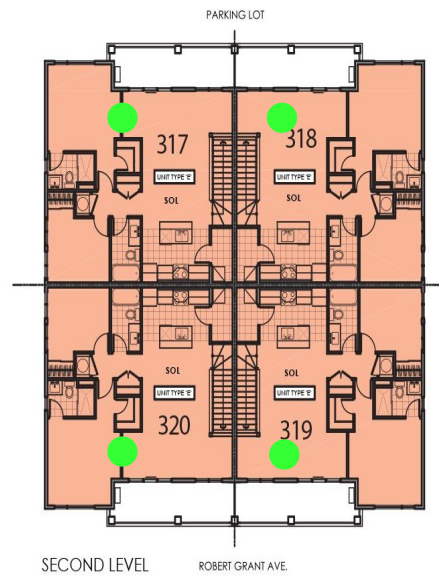
SECOND LEVEL
