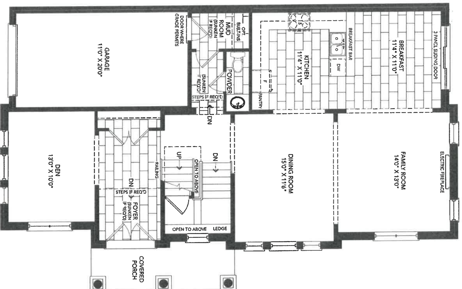
GROUND FLOOR PLAN ELEV. 1A1
