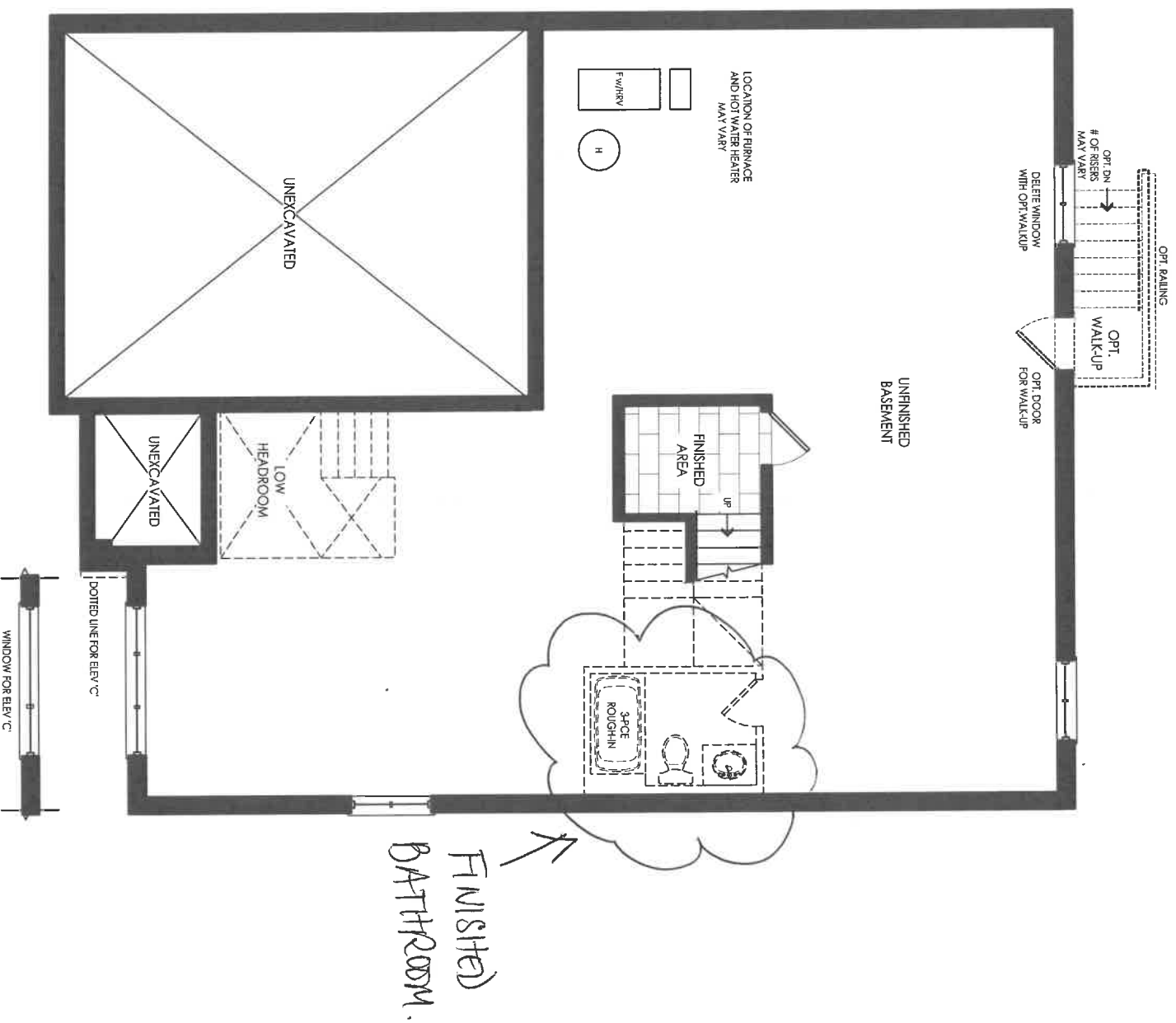
Elevation A, B & C Basement
