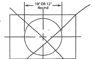
VP562/VP563 transition centers outlet over top of hood
