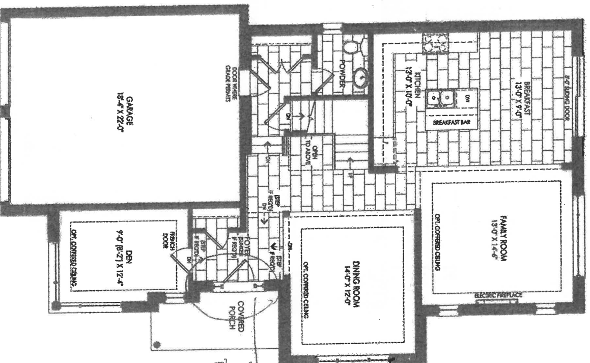
MAIN FLOOR ELEVATION C
