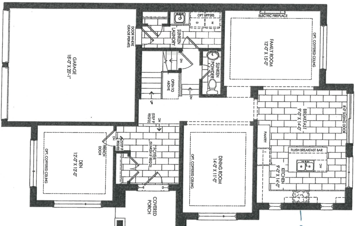
MAIN FLOOR ELEVATION C
