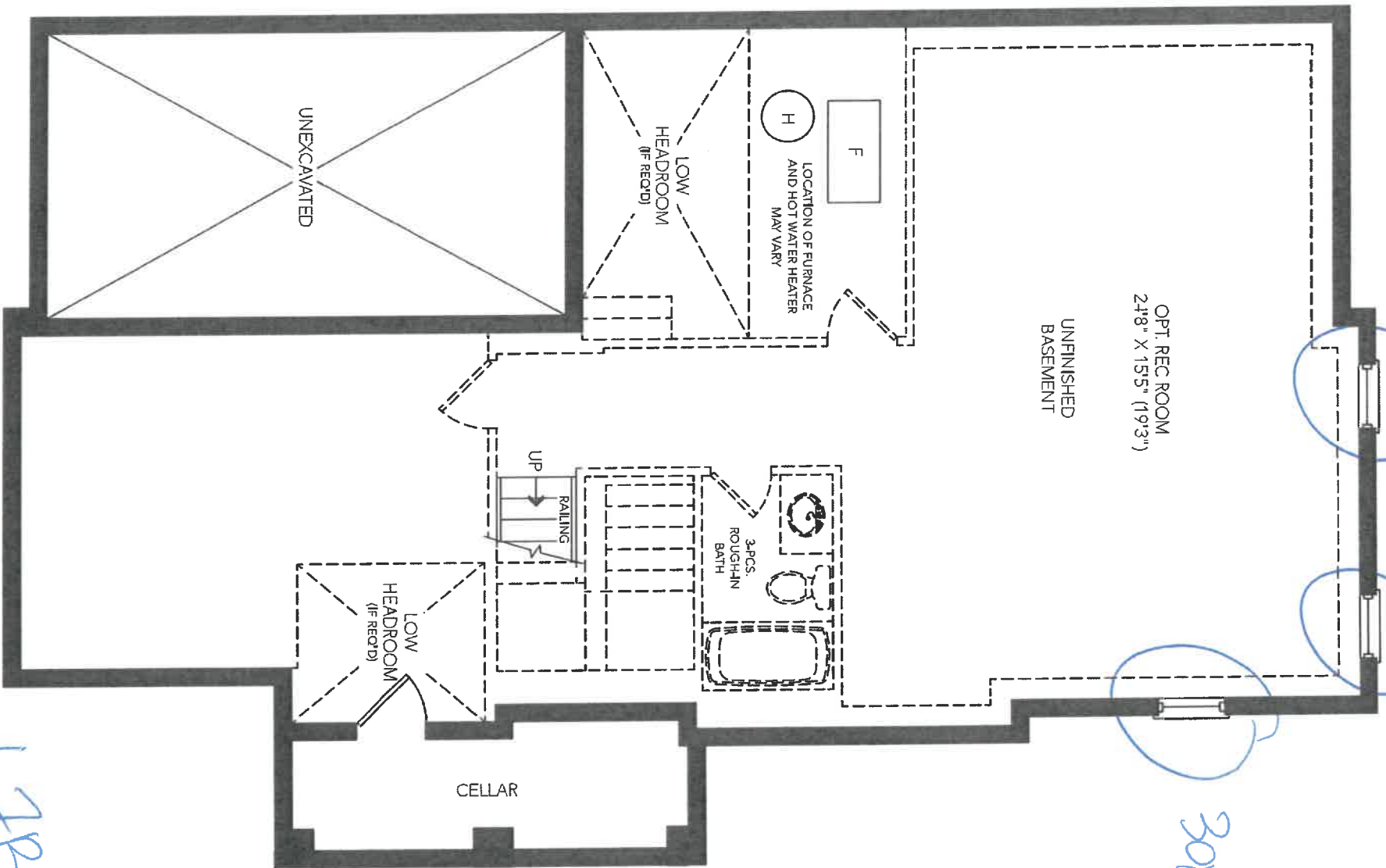
BASEMENT PLAN ELEV. 'A'
