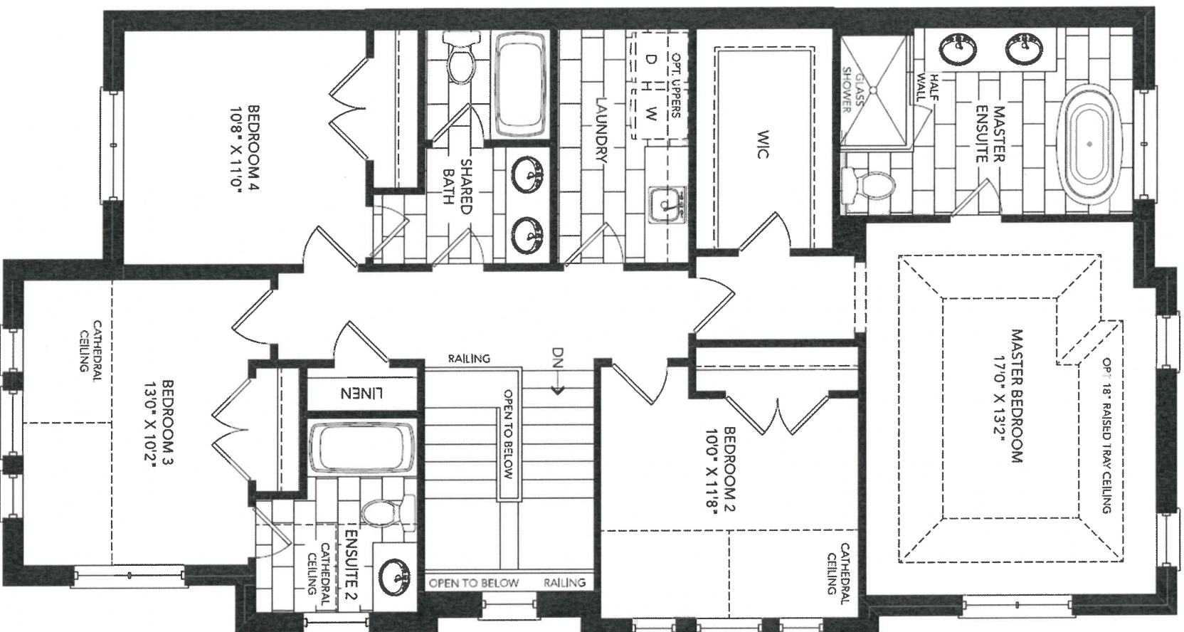
SECOND FLOOR PLAN ELEV. 'A'
