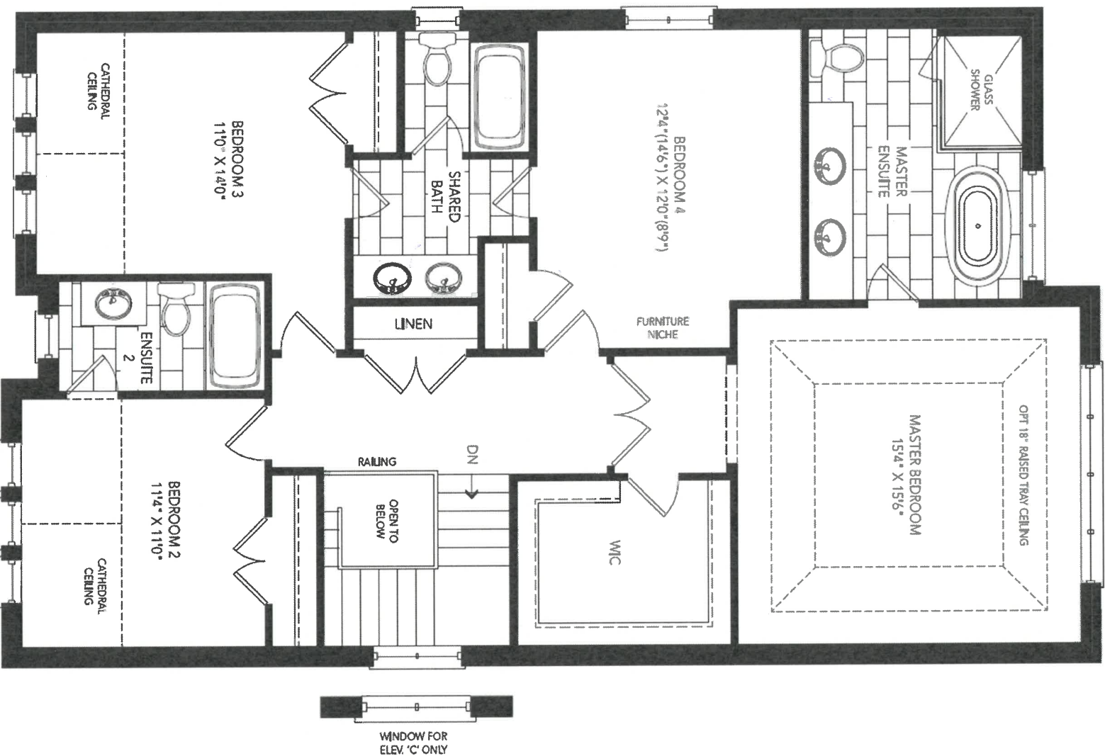
SECOND FLOOR PLAN ELEV. 'A'
