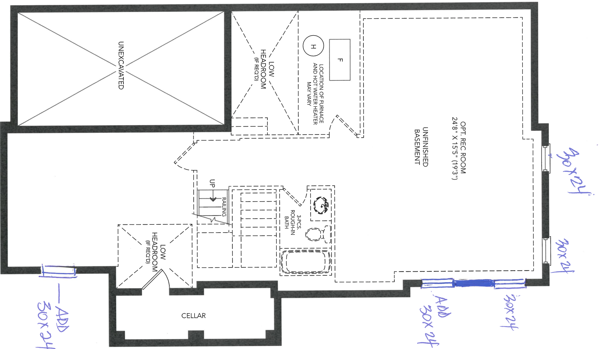
BASEMENT PLAN ELEV. 'A'
