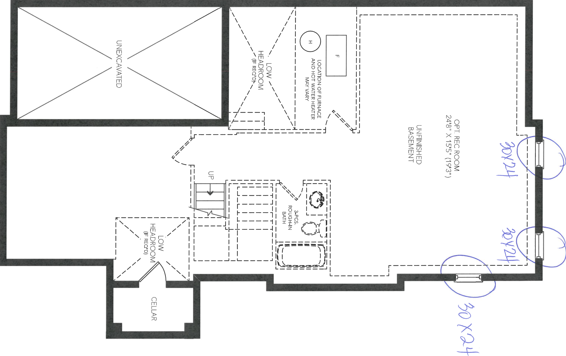
PARTIAL BASEMENT ELEV. 'B' & 'C'
