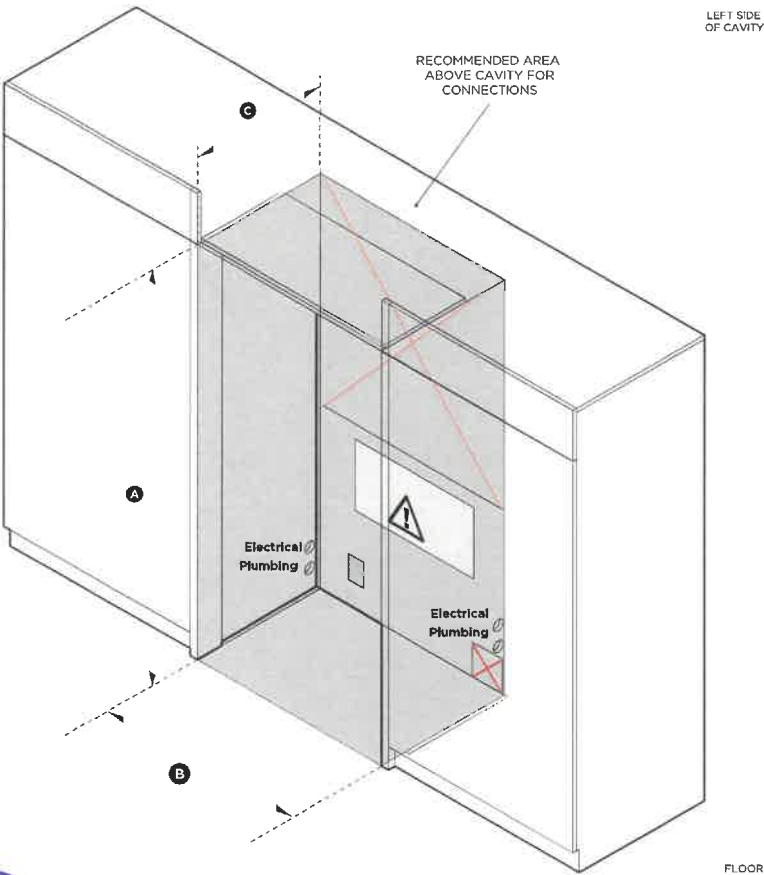
ISO VIEW OF CAVITY
