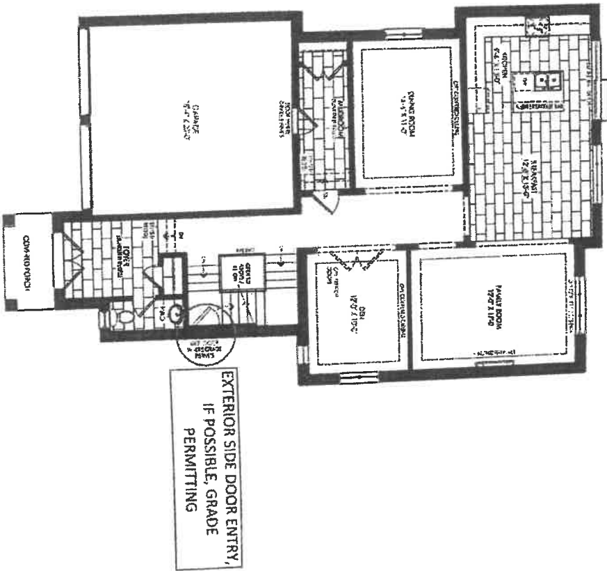
Elevation A Ground Floor
