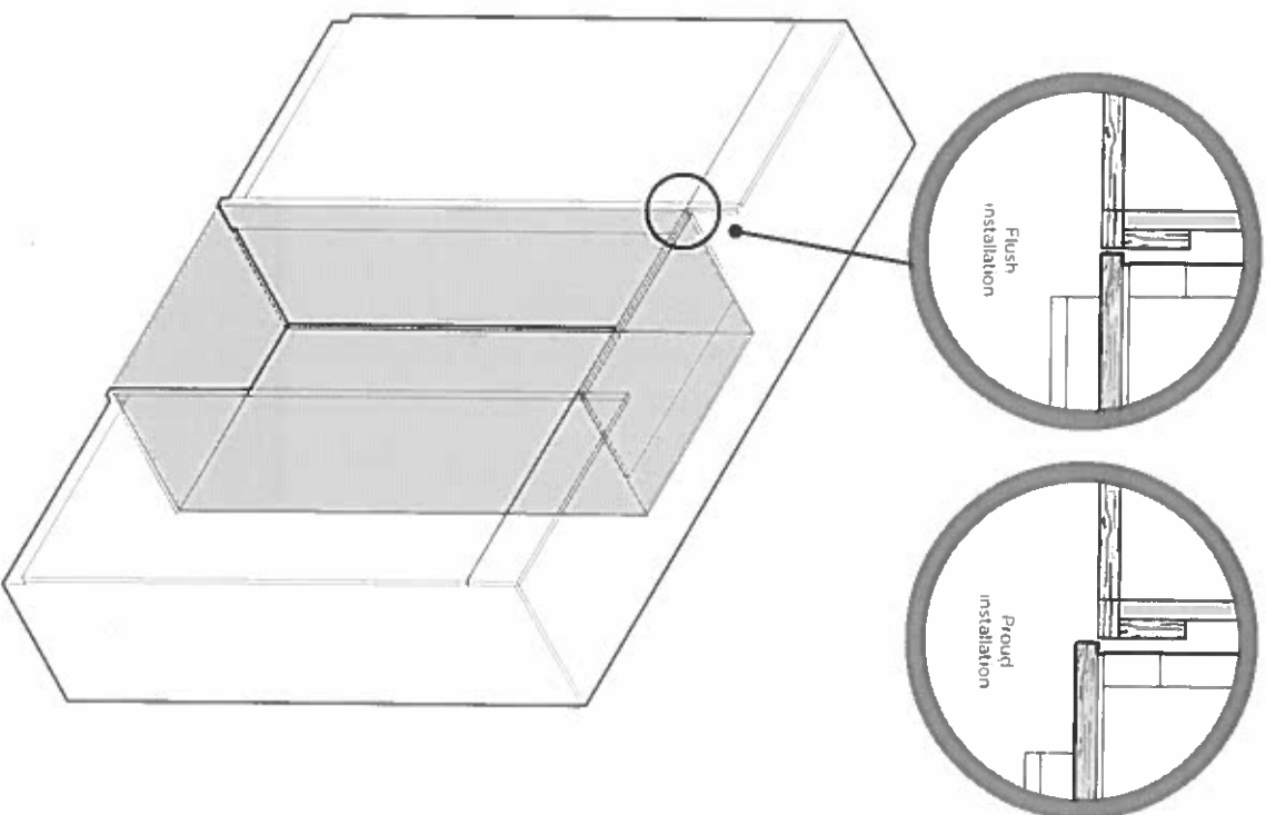
FRAMED CABINETRY (Aligns the appliance with the frame of the cabinetry)
