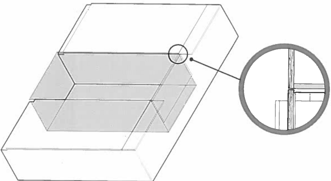
FRAMELESS CABINETRY (Aligns the appliance with the cabinetry)
