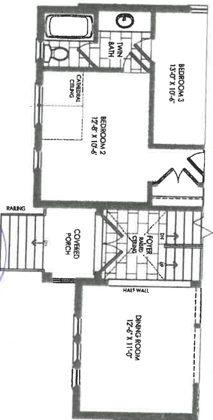
PARTIAL GROUND FLOOR ELEV. 'B'
