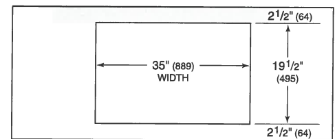
COUNTERTOP CUT-OUT
