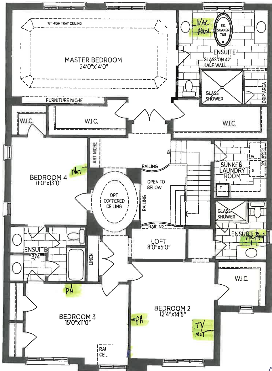
SECOND FLOOR EL. A
