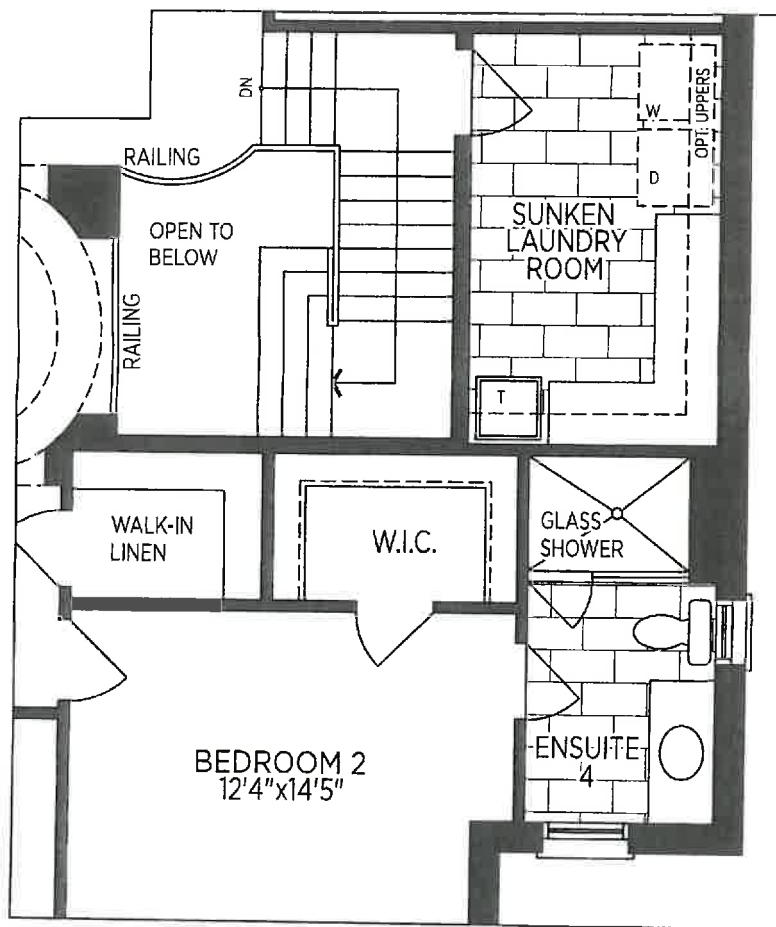
OPT. SECOND FLOOR EL. A/B
