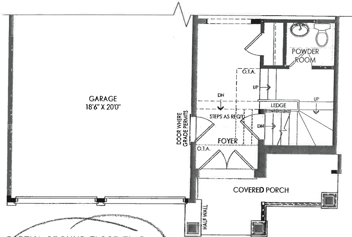
PARTIAL GROUND FLOOR EL. B
