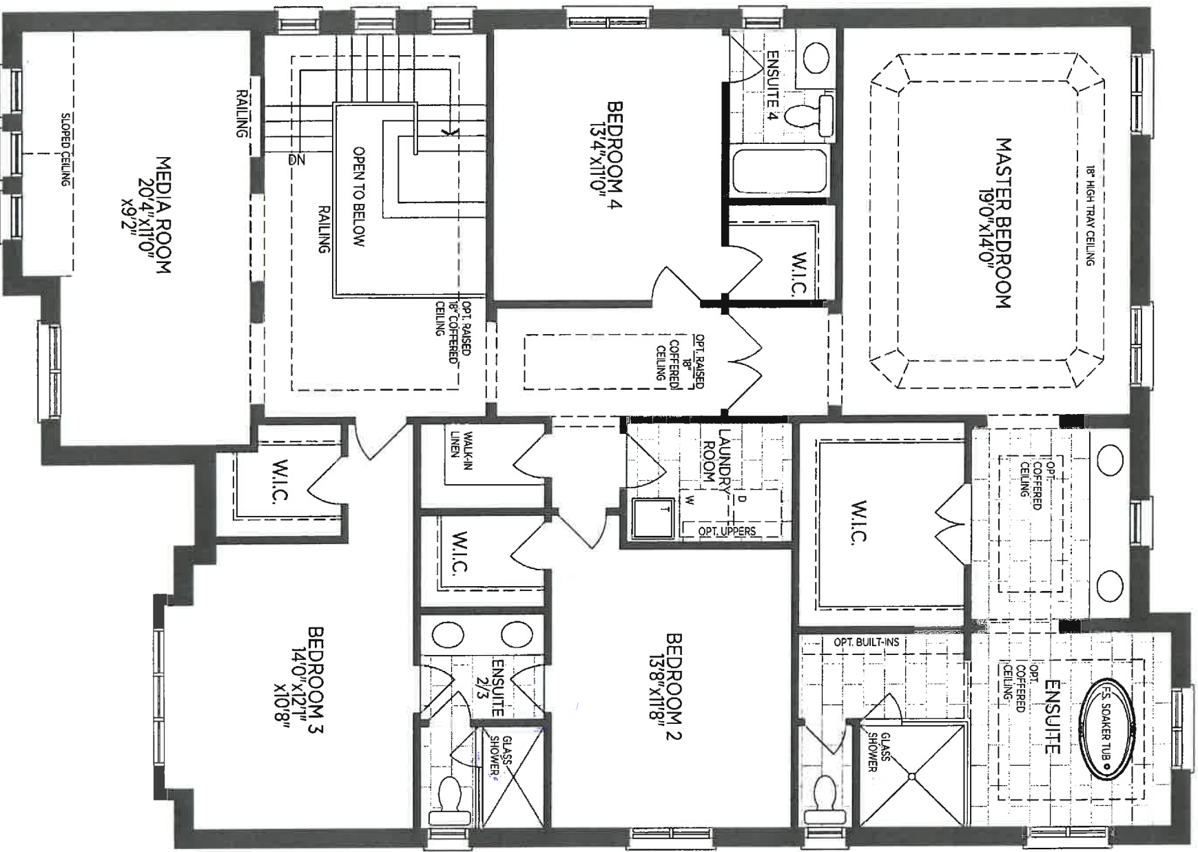
SECOND FLOOR EL. B
