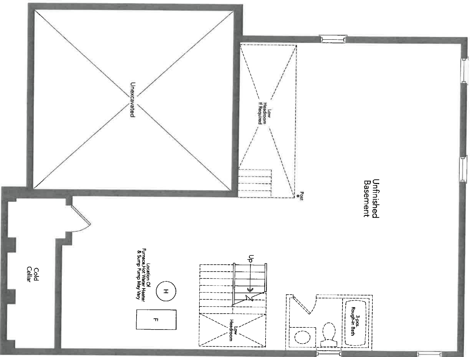
Basement Elevation A
