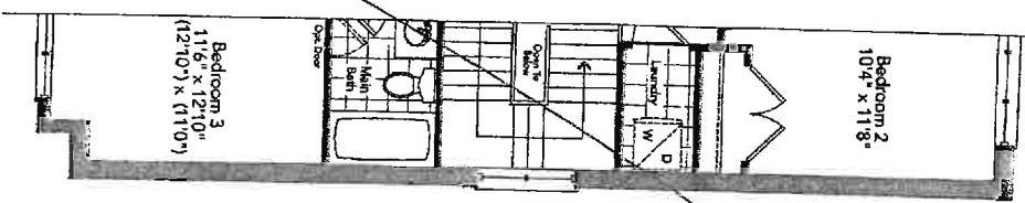
Partial Optional Second Floor Elevation B
