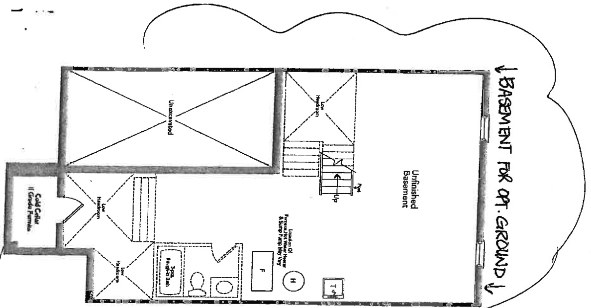
Basement Elevation A & B
