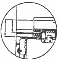
2 7/8" (73mm) - 4" (102mm) toe kick clearance measured from rear of door panel
