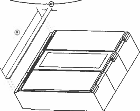
TRIPLE INSTALL
