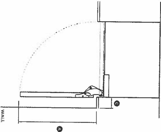
90° DOOR OPENING
