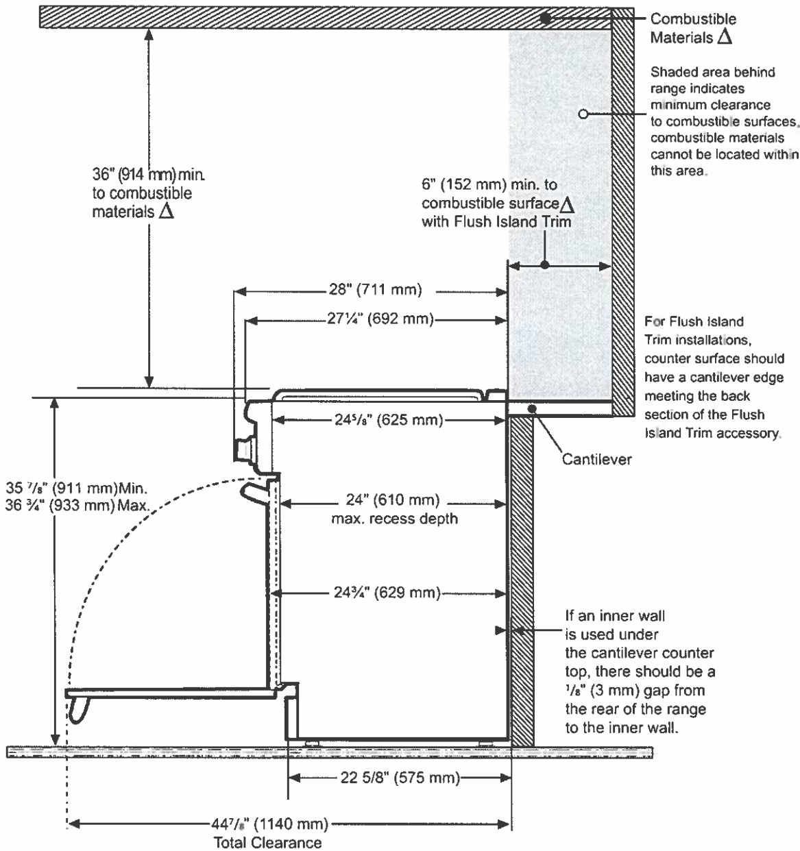
36-INCH RANGE DIMENSIONS AND CLEARANCE REQUIREMENTS WITH "FLUSH ISLAND TRIM"
