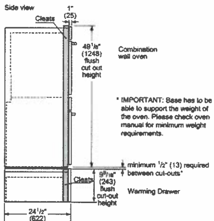
Flush installation
