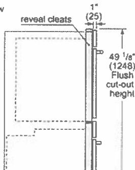
Standard Installation
