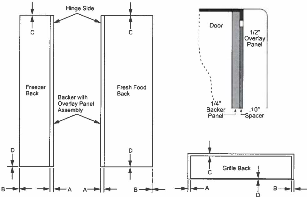
PANEL DIMENSIONS
