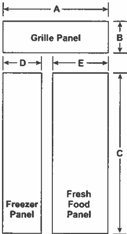
PANEL DIMENSIONS
