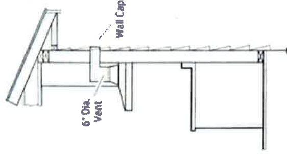
Wall Venting
