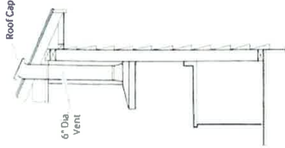
Roof Venting
