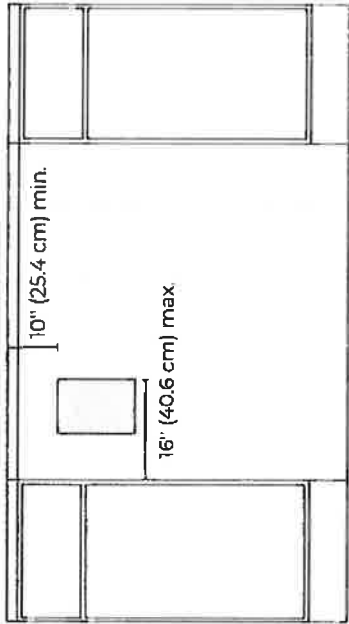
RECOMMENDED ELECTRICAL OUTLET ZONE
