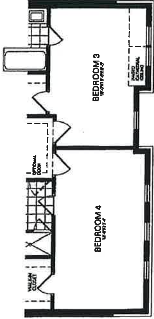
PARTIAL SECOND FLOOR - ELEVATION C TYPE OAK-432
