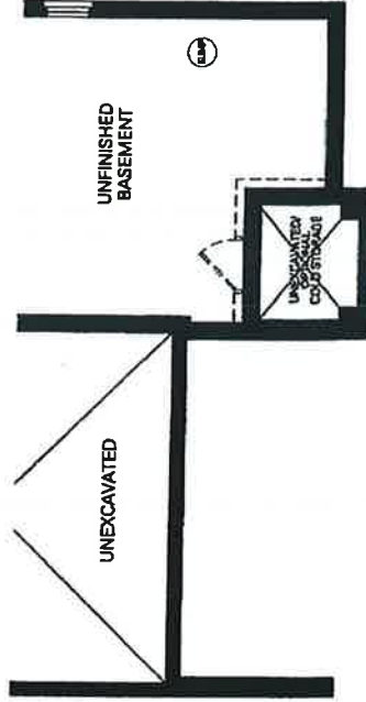
PARTIAL BASEMENT - ELEVATION C TYPE OAK-432
