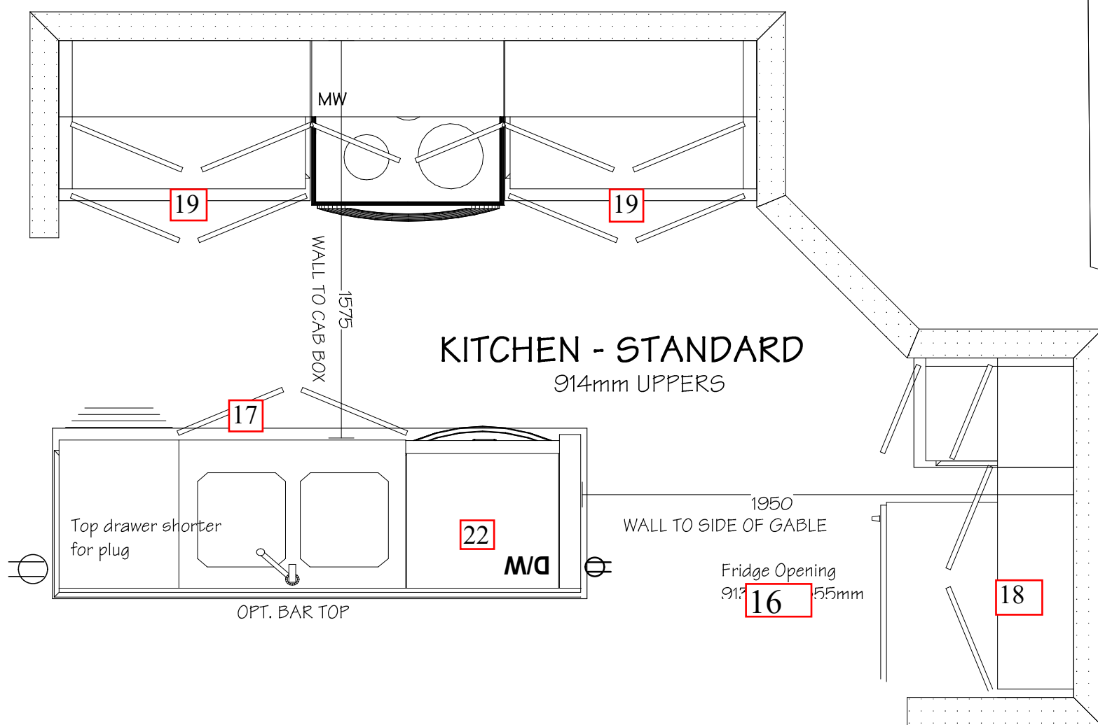
ITEM #2 - Standard Kitchen Layout - Level 1 Cabinetry
