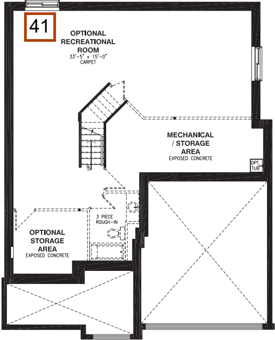
BASEMENT FLOOR - ELEVATION A
