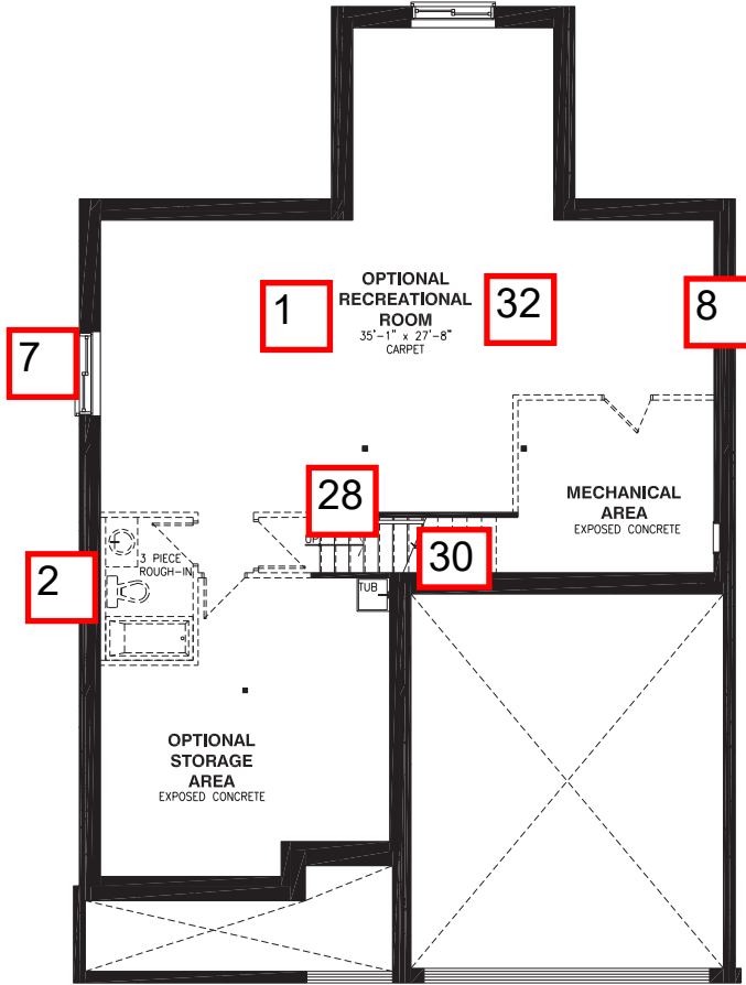
BASEMENT FLOOR
