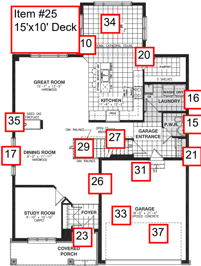
GROUND FLOOR - ELEVATION A
