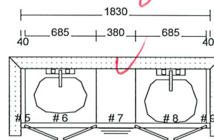
OPT 4PC ENSUITE 2ND FLOOR
