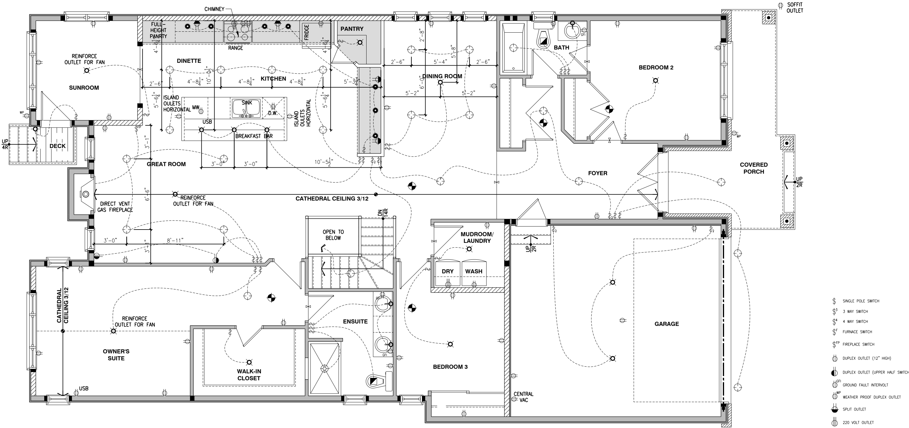
ELECTRICAL PLAN - GROUND FLOOR - STANDARD KITCHEN - SUNROOM UPGRADE - 4 PC ENSUITE UPGRADE - ELEVATION A
