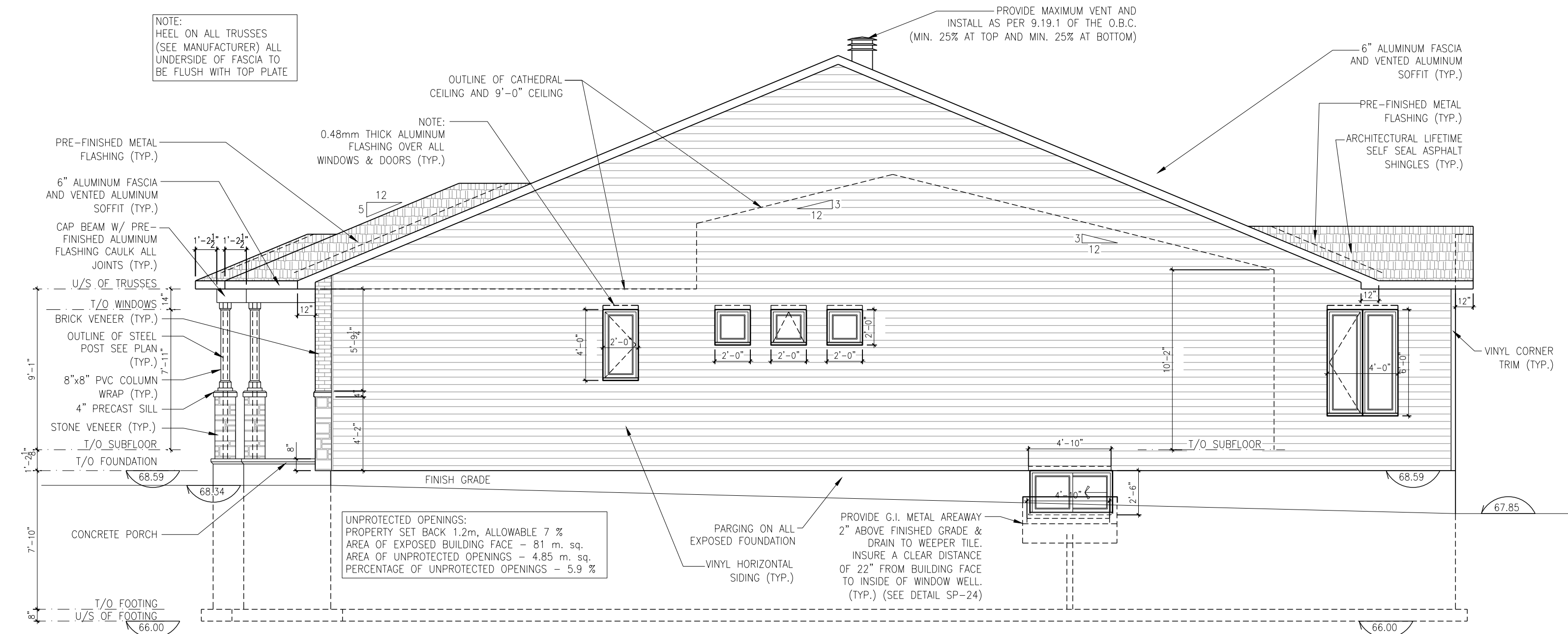
RIGHT ELEVATION - SUNROOM UPGRADE - ELEVATION A
