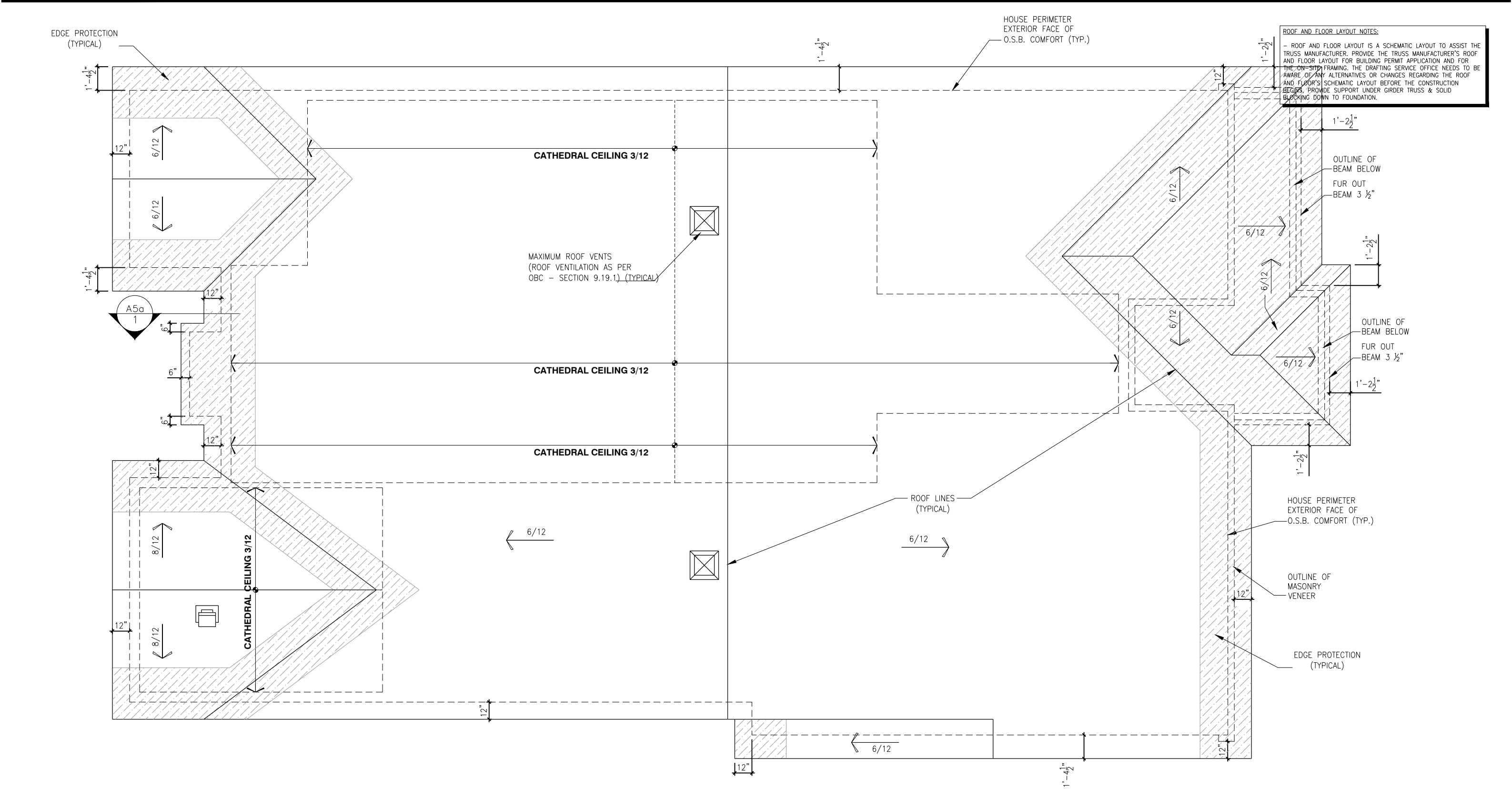
ROOF PLAN - SUNROOM UPGRADE - ELEVATION A
