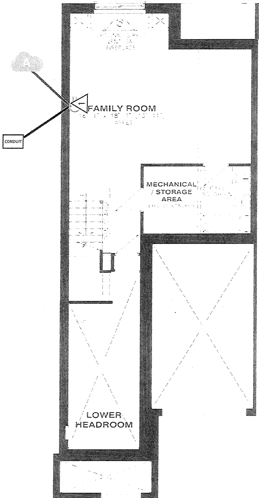
BASEMENT FLOOR
