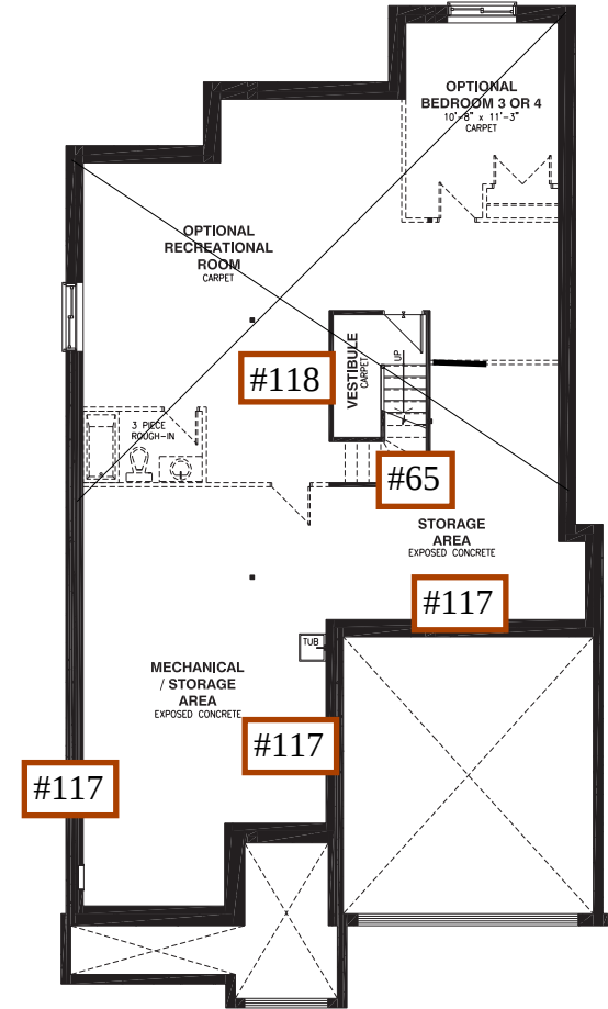
BASEMENT FLOOR - ELEVATION A
