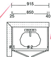
MAIN - 2ND FLOOR
