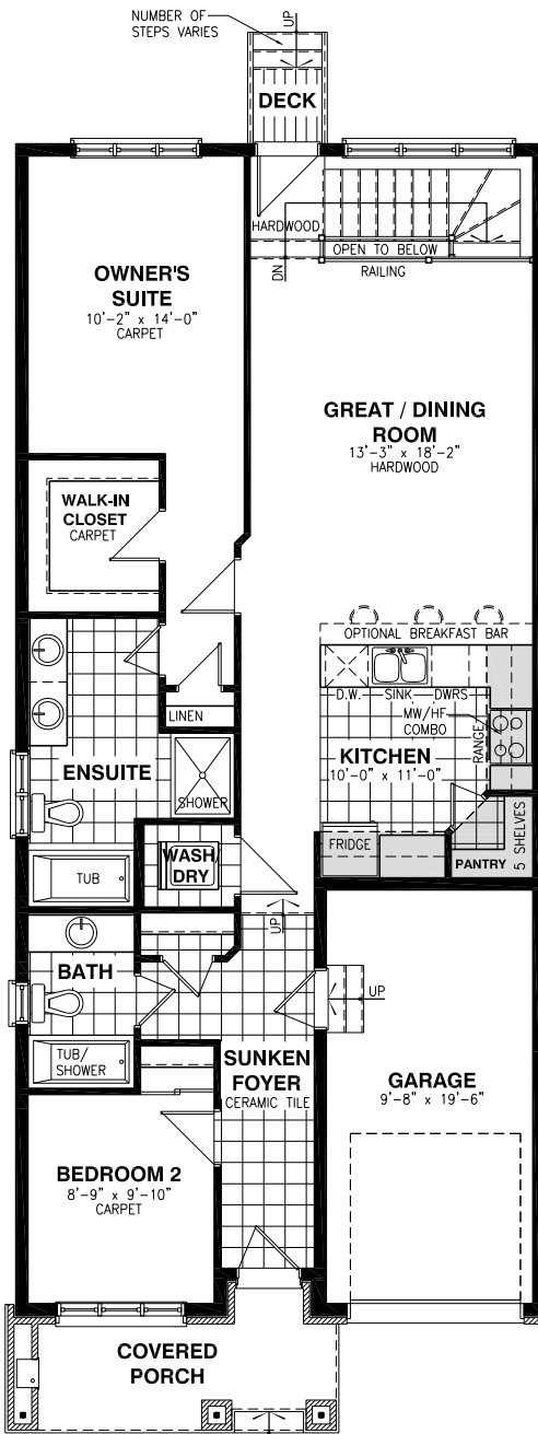
GROUND FLOOR PLAN OPTIONAL 2 BEDROOM
