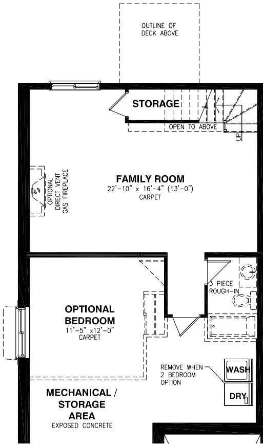
WALKOUT BASEMENT WHERE APPLICABLE
