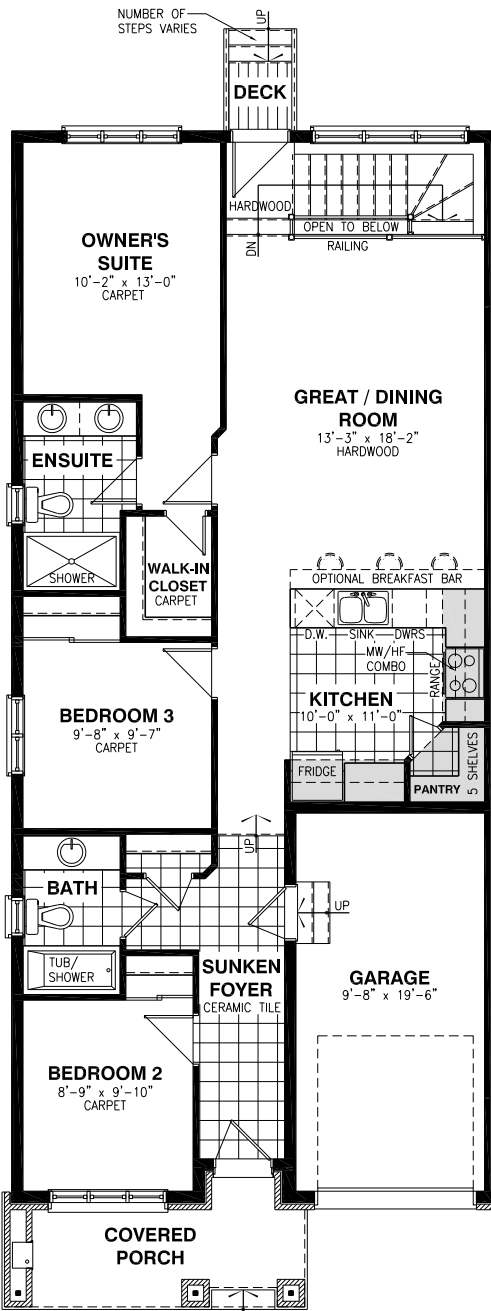
GROUND FLOOR PLAN STANDARD 3 BEDROOM
