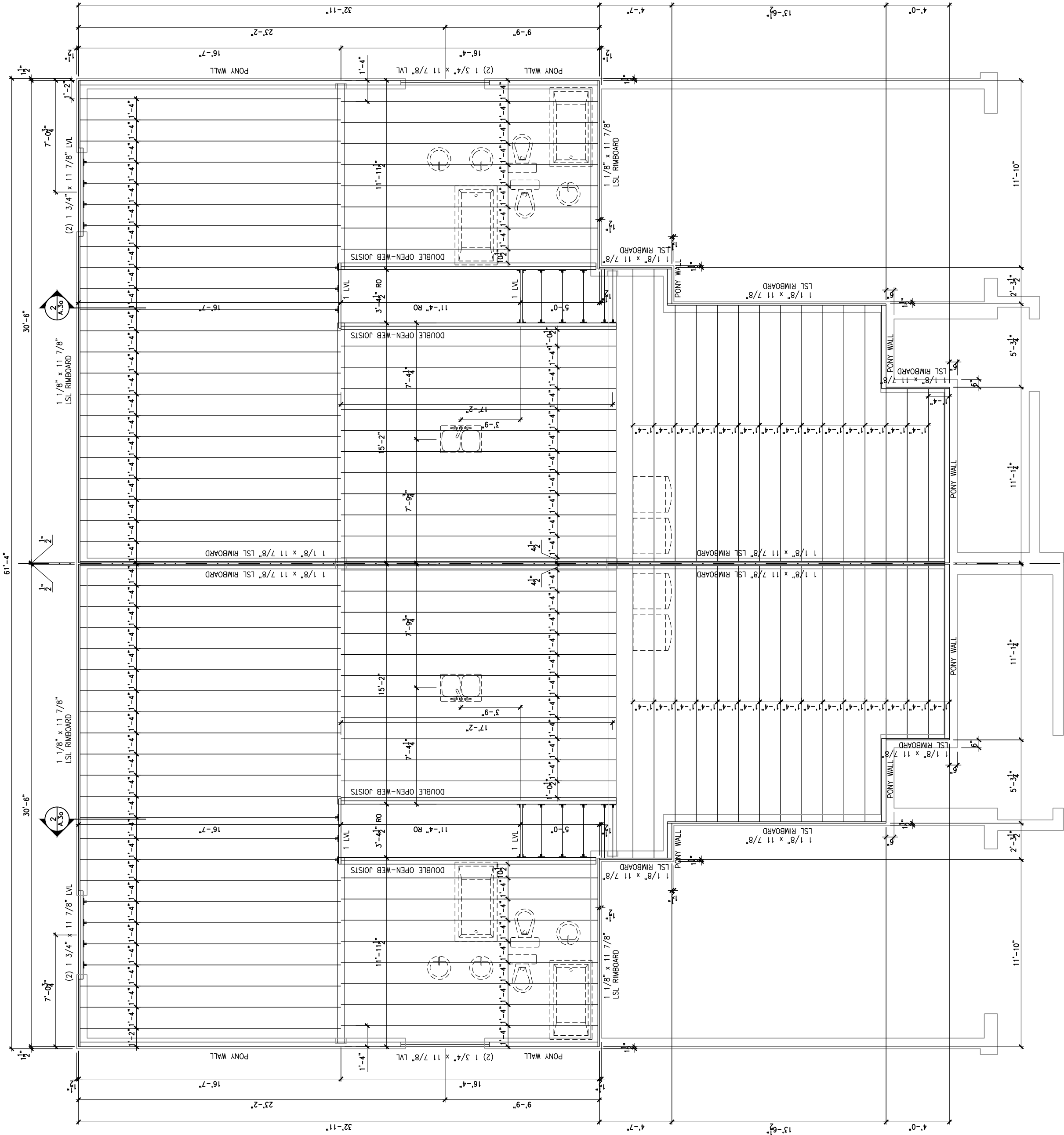
1 A.6a GROUND FLOOR - FLOOR JOIST FRAMING PLAN SCALE: 3/16" = 1'-0"
