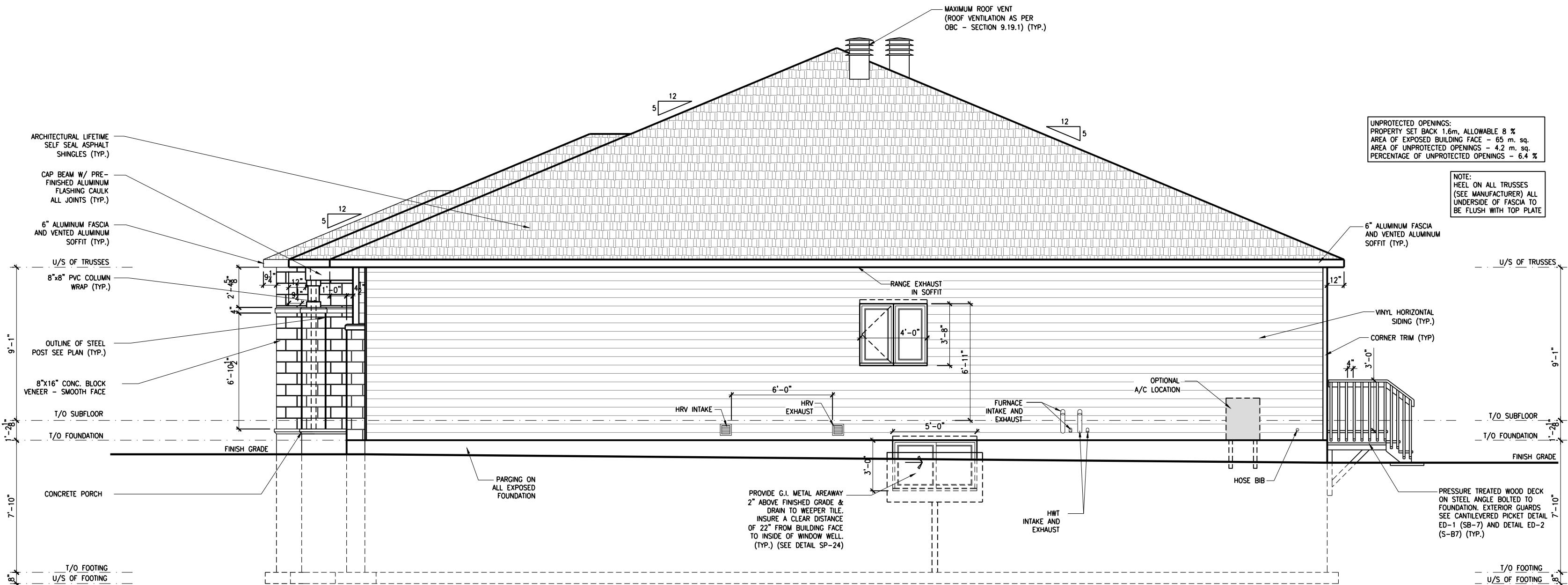
1 LEFT SIDE ELEVATION A.2a SCALE: 3/16" = 1'-0"
