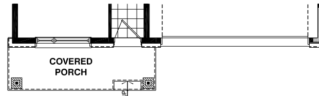
Ground Floor - 3 Bedroom - Elevation B
