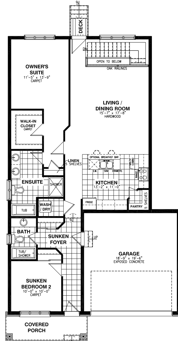
Ground Floor - Optional 2 Bedroom - Elevation A
