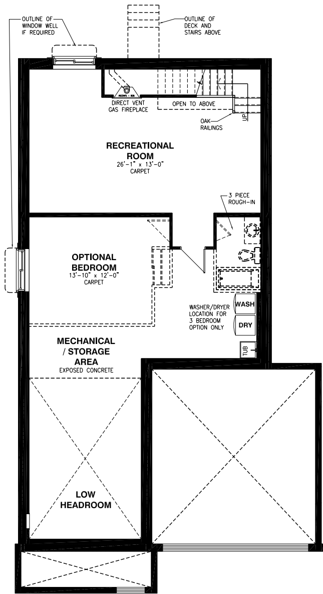
Basement Floor - Elevation A and B
