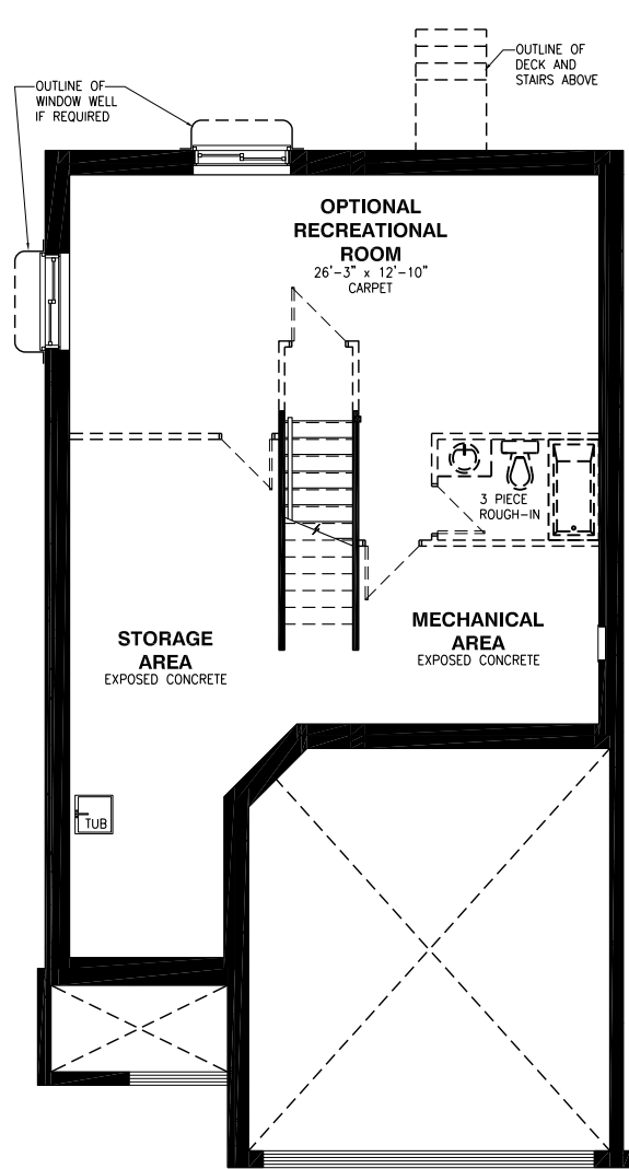
Basement Floor
