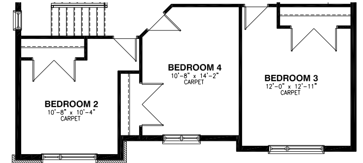
Second Floor - Elevation B
