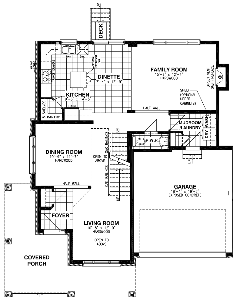
Ground Floor - Elevation Corner Lot
