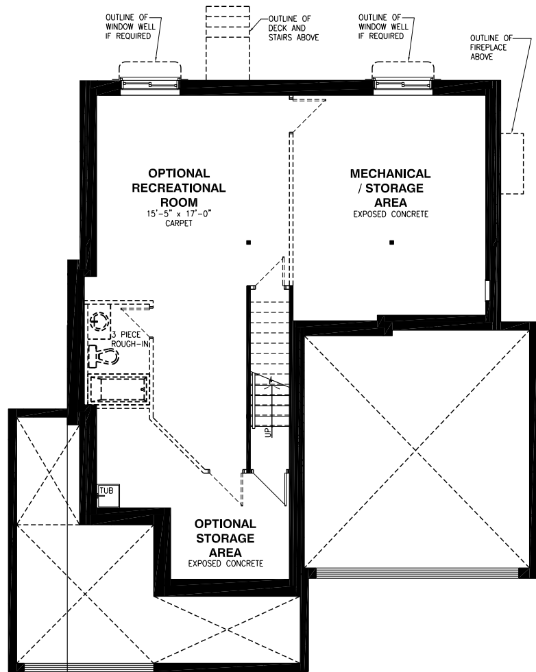
Basement Floor - Elevation Corner Lot
