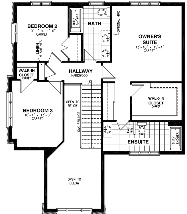
Second Floor - Elevation Corner Lot
