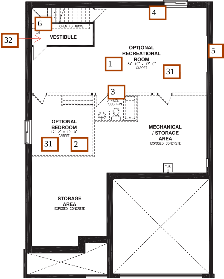
BASEMENT FLOOR - ELEVATION A
