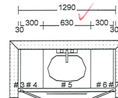
OPT 4PC ENSUITE 2ND FLOOR - FLOATING VANITY - Install 314mm from floor
