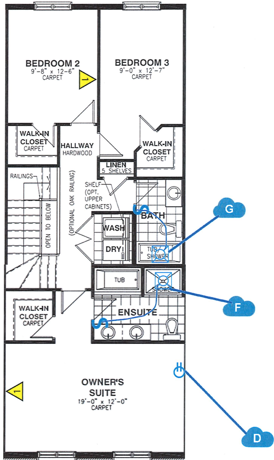
SECOND FLOOR
