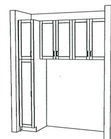
OPT LAUNDRY 750mm UPPERS INSTALL CABS 1475mm FROM FINISHED FLOOR
