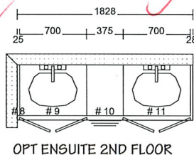
OPT ENSUITE 2ND FLOOR
