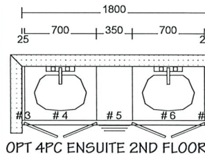
OPT 4PC ENSUITE 2ND FLOOR
