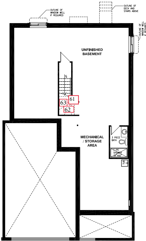
Basement Floor
