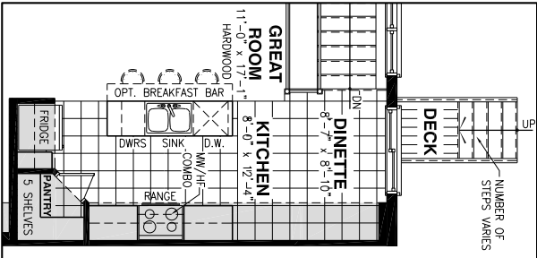
OPTIONAL KITCHEN #1
